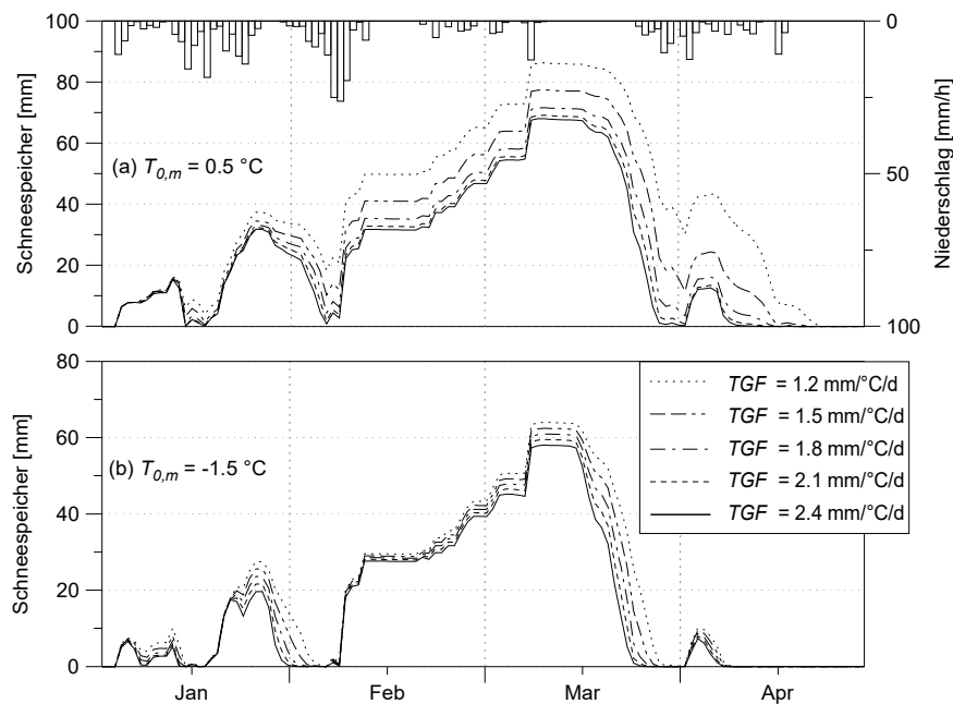
Figure 4.14.3: temporal course of snow water equivalent for different degree day factors: (a) melt threshold temperature T_{0,m} = +0.5 \text{ }^{\circ}\text{C} , (b) T_{0,m} = -1.5 \text{ }^{\circ}\text{C} , Rietholzbach basin, 1984; “Schneespeicher” means snow water equivalent, “Niederschlag” means precipitation
