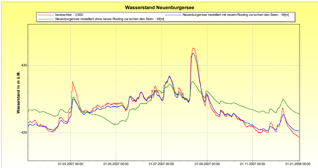
Figure 2.18.5: Example for modeled lake water table with and without the new hydraulic connection abstraction rule (red=observed water table, green=modeled water table without hydraulic connection, i.e. classic one-way-routing, and blue=modeled water table with hydraulic connection)
