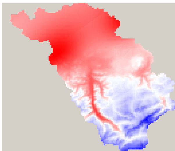
Figure 2.3.17: interpolation results for IDW (North) and EDR (South) with 10km transition-range
