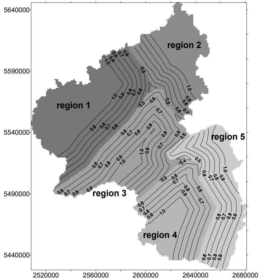
Figure 2.3.12: Weighting of the actual region if using multiple regions. Rheinland-Pfalz, Germany, 5 regions, maximum transition distance r was set to 20 km.
