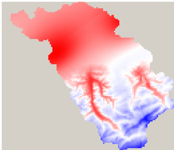
Figure 2.3.16: interpolation results for IDW (North) and EDR (South) with 5km transition-range
