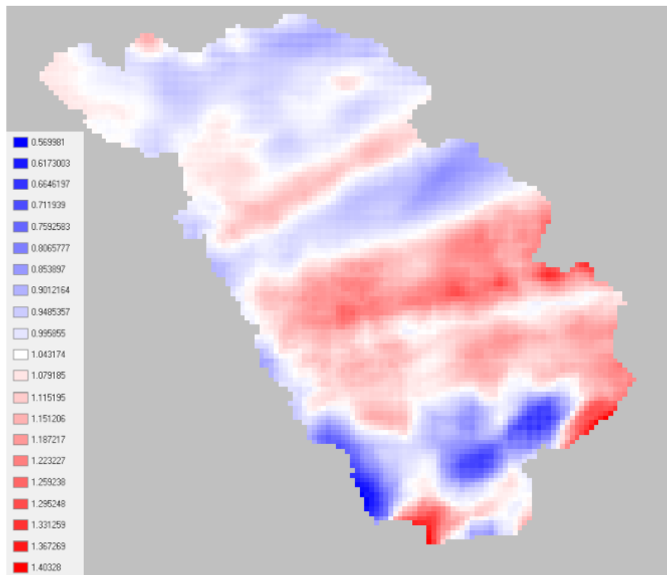
Figure 2.3.10: Sample correction factor grid for radar data for the river Thur basin
