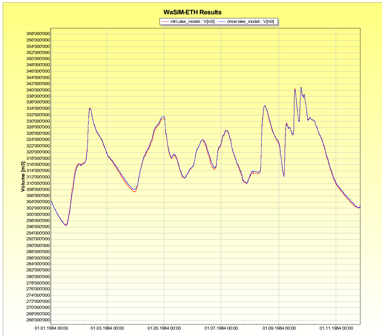
Figure 2.18.6: comparison of lake volume with the fully integrated lake model and with the simple (routing module only) lake model
