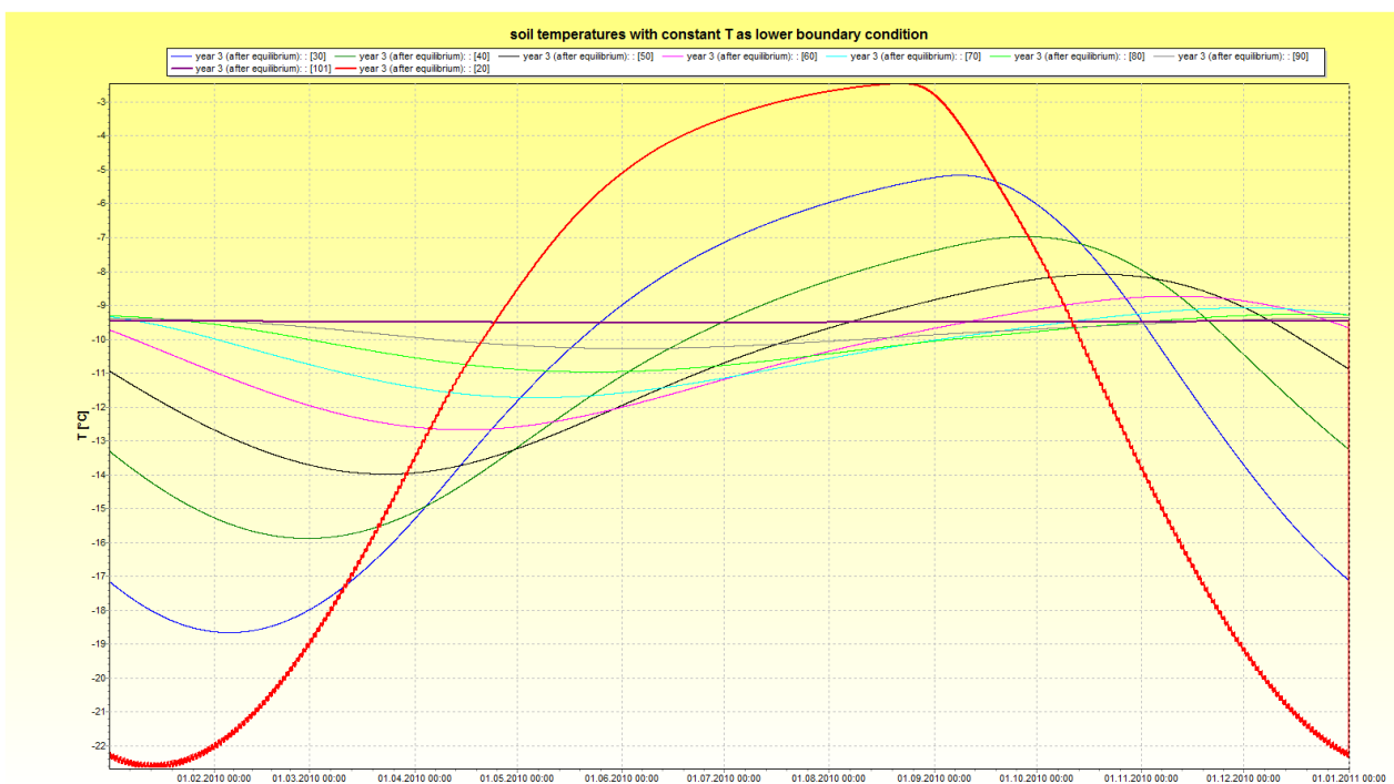
Figure 2.24.16: soil temperatures as time series for constant T lower boundary condition (red = 0.7m, blue = 1.7m, green = 2.7m, black = 3.7m etc. down to 8.8m for violet)
