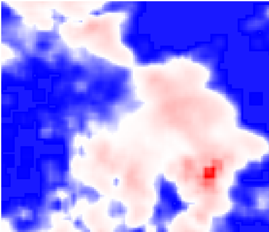
Figure 2.3.9: interpolated region of interest, mapped to precipitation values
