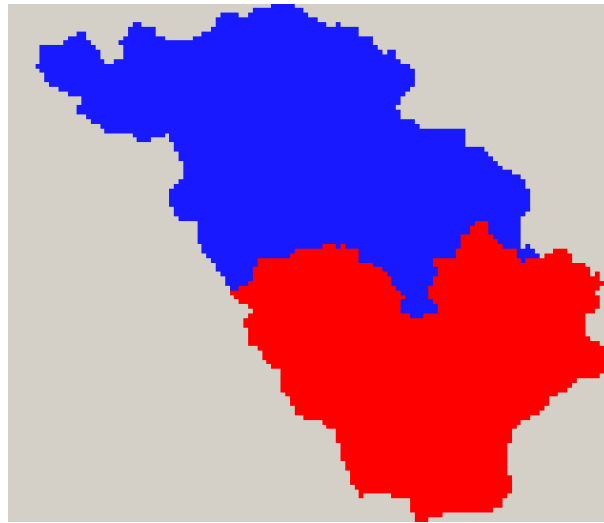
Figure 2.3.13: Definition of two regions for the river Thur basin (Switzerland, 1700km 2 ), the entire grid encompasses an area of 65.5 km x 56 km, each cell is 500 by 500m (also for all following figures)
