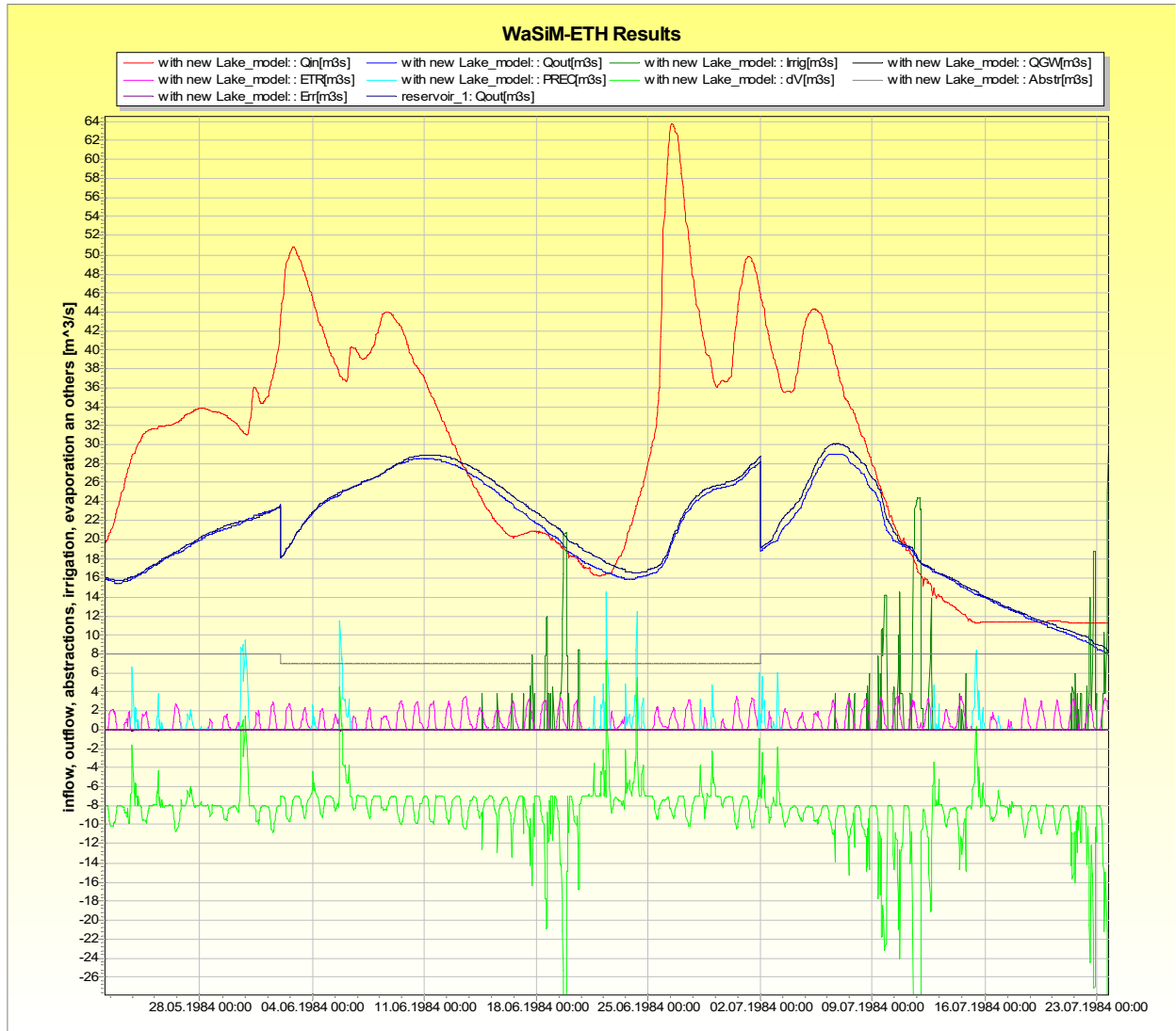
Figure 2.18.7: some components of the lakes water balance statistics.
