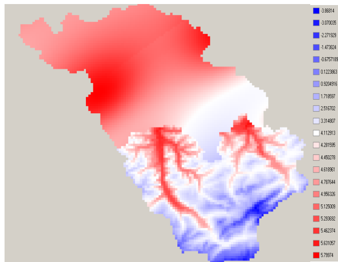
Figure 2.3.14: interpolation results for IDW (North) and EDR (South) without smooth transition
