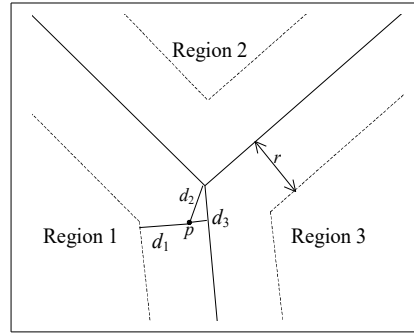
Figure 2.3.11: Weighting of multiple regions for a point p near the regions crossing point
