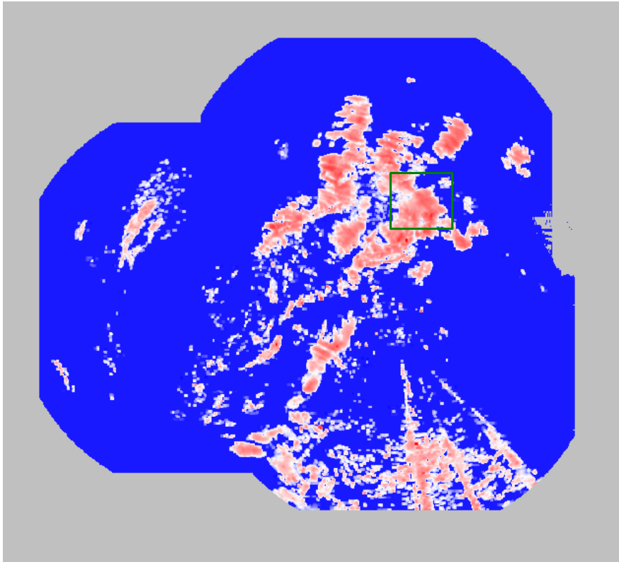
Figure 2.3.8: Example for a Swiss radar data image covering entire Switzerland with three radar stations (unmapped values)
