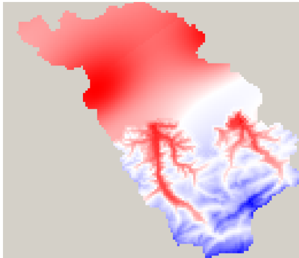
Figure 2.3.15: interpolation results for IDW (North) and EDR (South) with 1km transition-range
