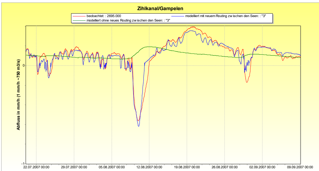
Figure 2.18.4: example for flow reversals between lakes Bielersee and Neuenburgersee due to the new abstraction rule as hydraulic connection
