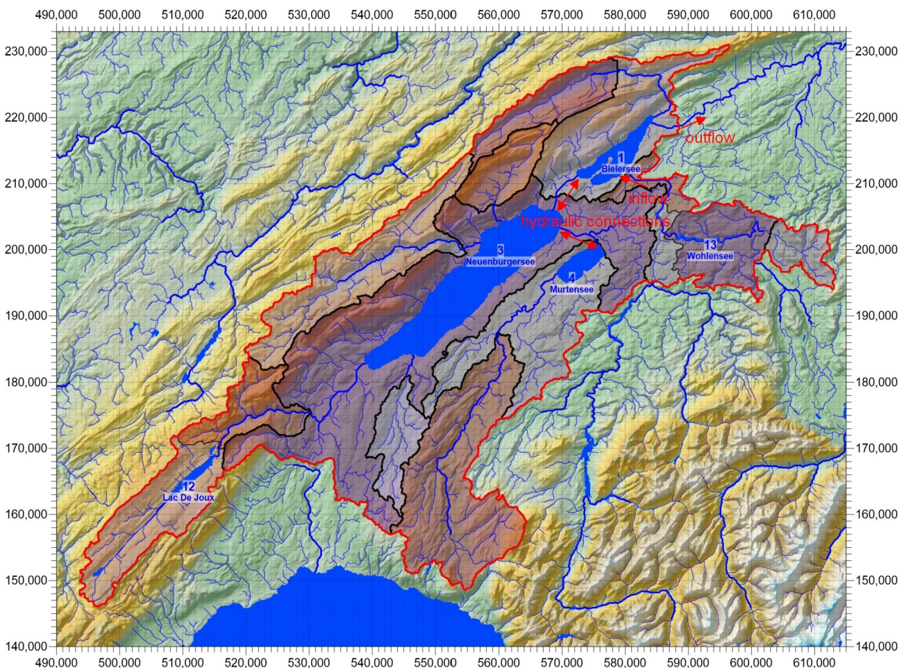
Figure 2.18.3: example for hydraulic connections between three lakes
